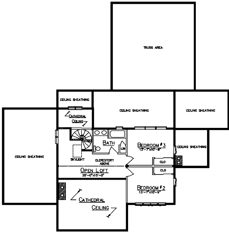
CLERESTORY PLAN
