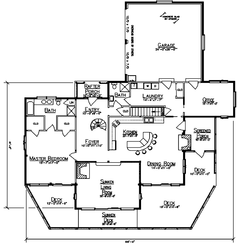
FLOOR PLAN
