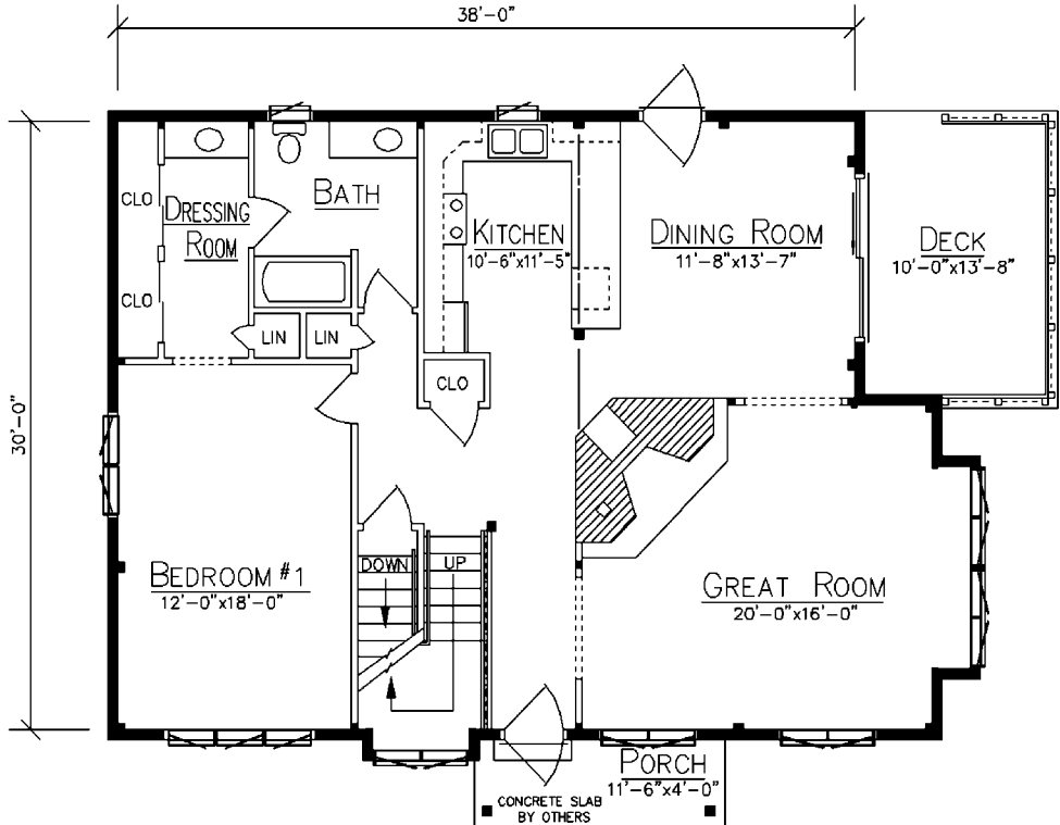
FLOOR PLAN
