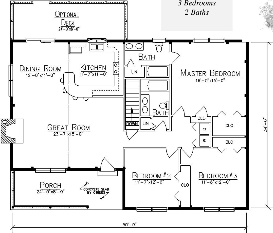
FLOOR PLAN
