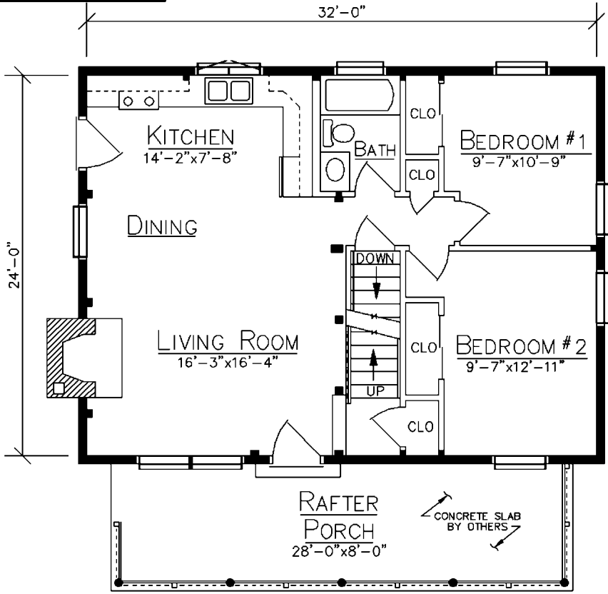
FLOOR PLAN
