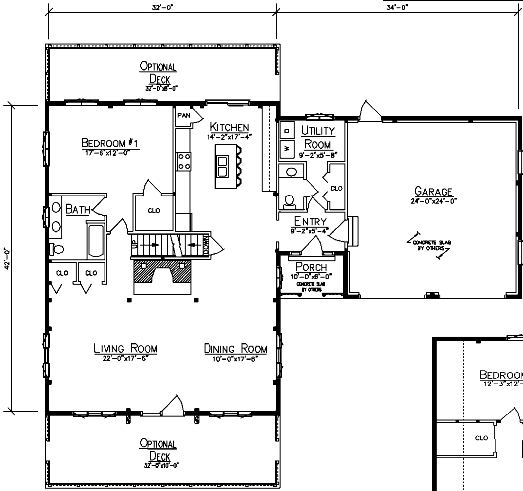
FLOOR PLAN
