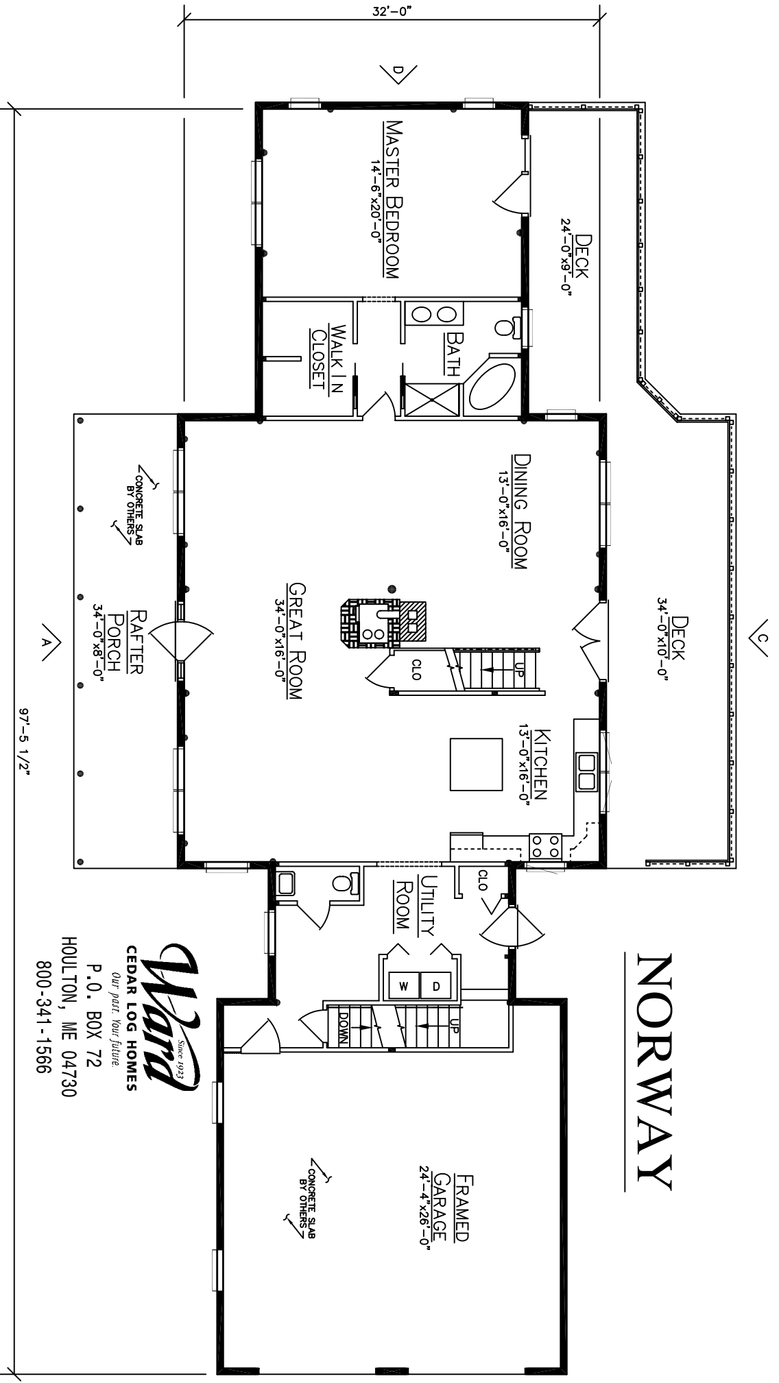
FLOOR PLAN
