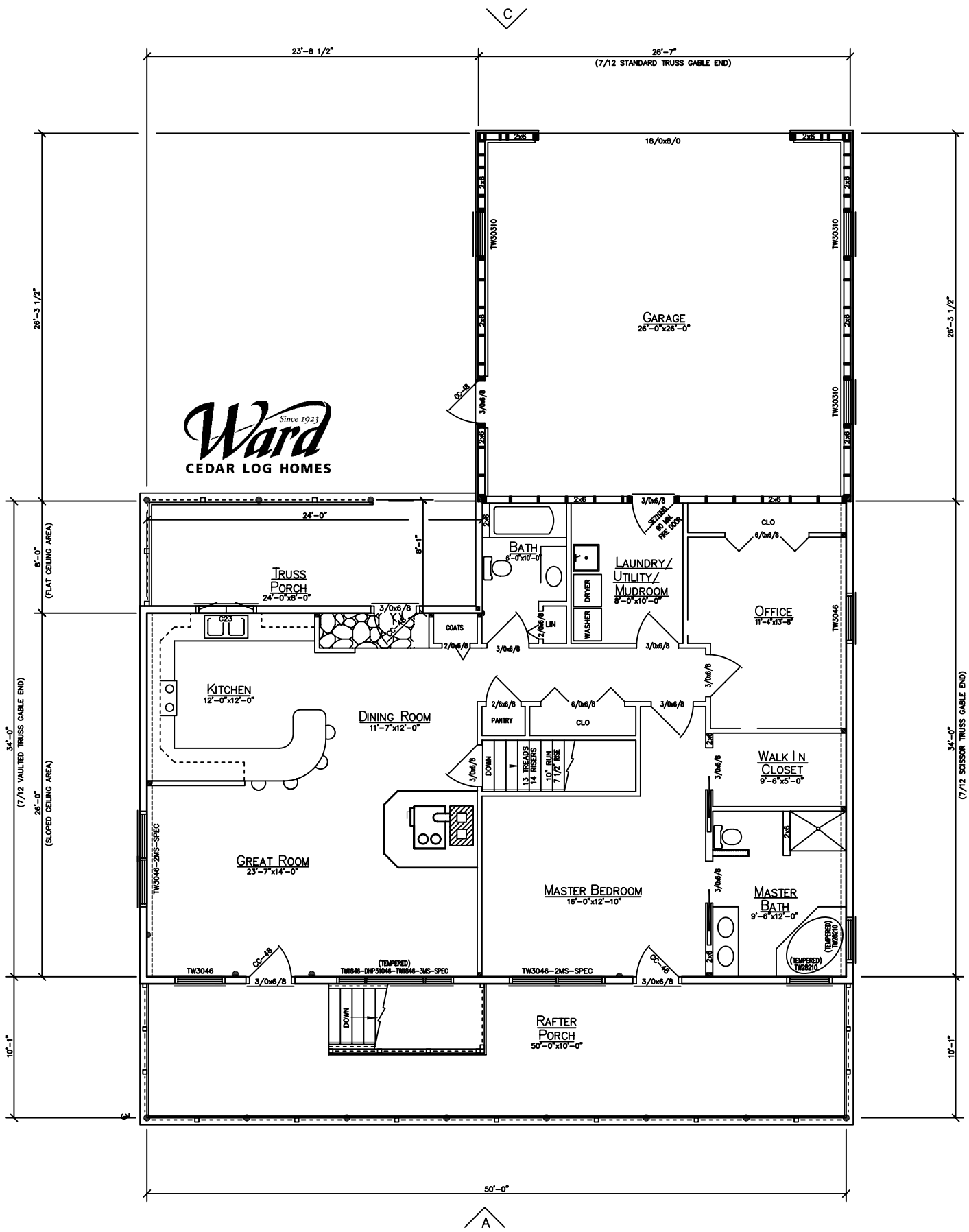
FLOOR PLAN
