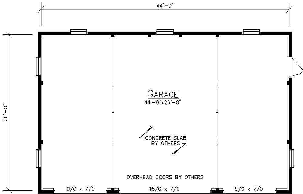
FLOOR PLAN
