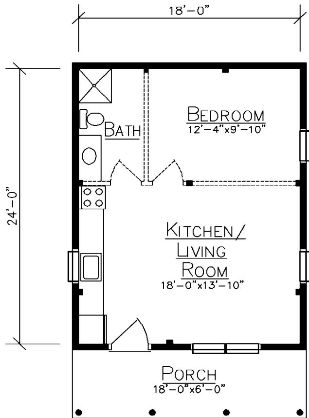
FLOOR PLAN
