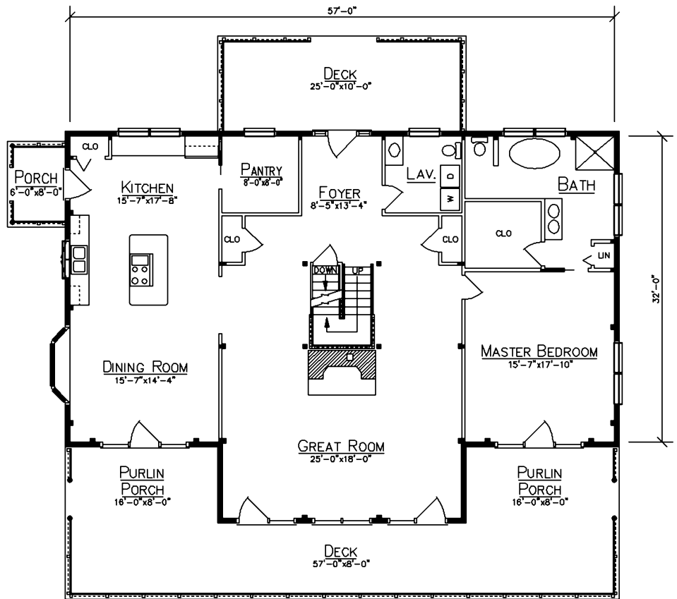
FLOOR PLAN
