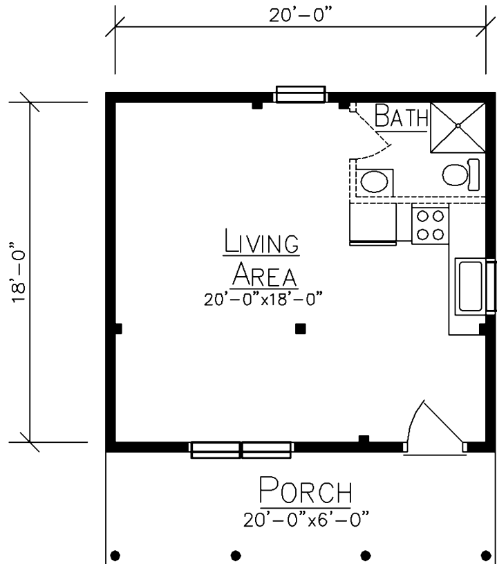
FLOOR PLAN
