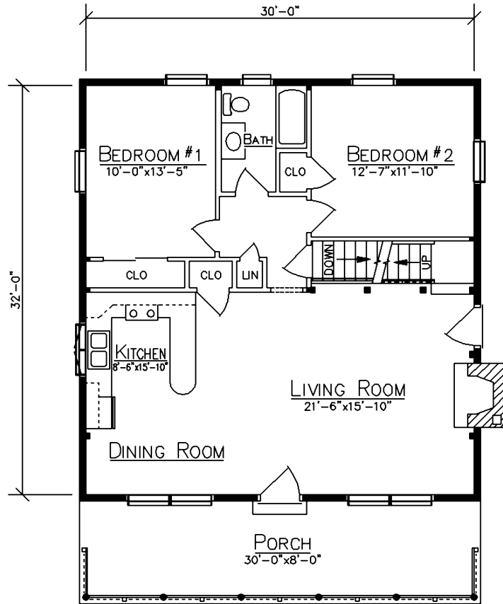
FLOOR PLAN
