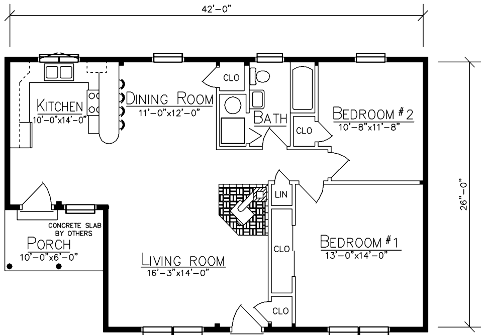
FLOOR PLAN
