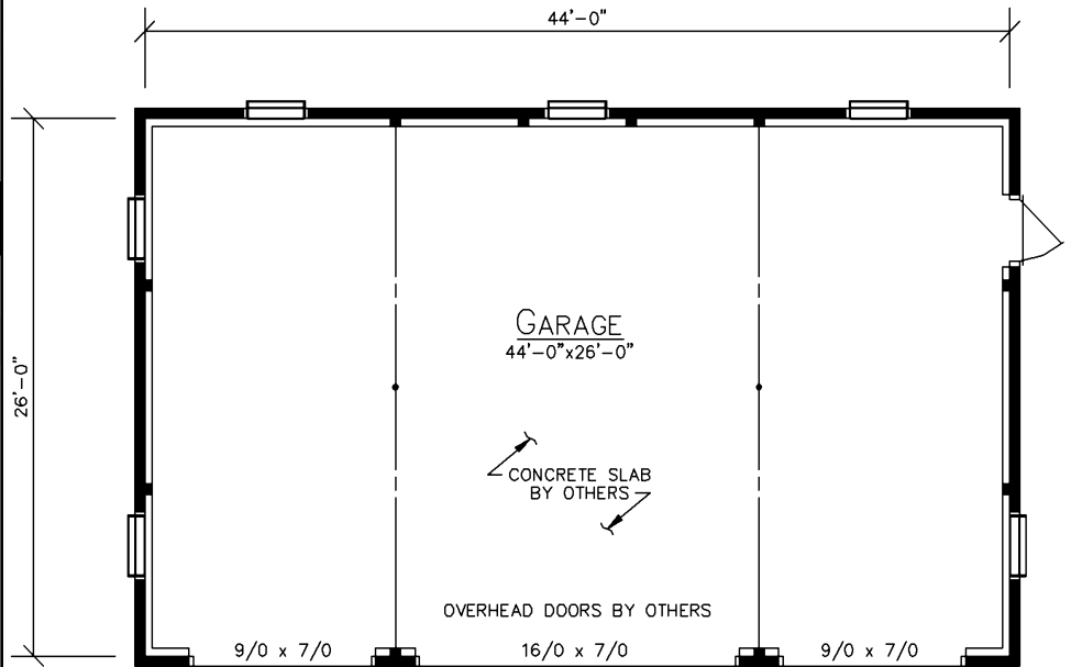
FLOOR PLAN
